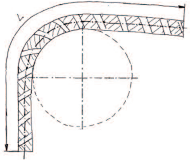
Push/Pull Cable made by RINGSPANN RCS
